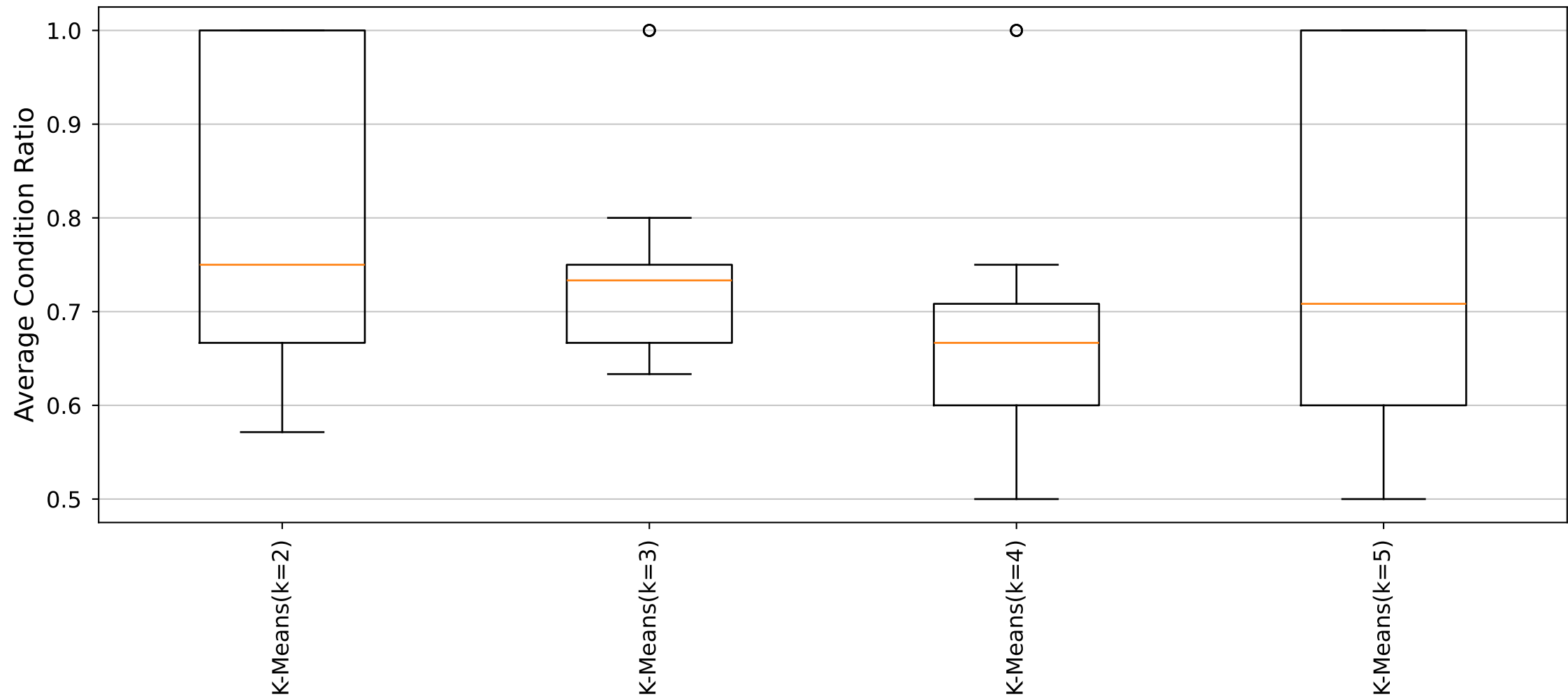
YARA Rules Average Condition Ratio Distribution (Cluster39_Size5 dataset)
